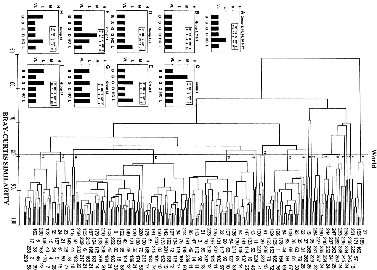
Fig. 3 Bray-Curtis similarity index dendrogram. Site numbers are shown adjacent to the branch tips and correspond to locations in Table 2. When 'cut' at the similarity level of 79, there are seventeen groups (numbers shown on cluster stems). These groups were further combined (see text) to create ranked abundance plots (small boxes A–I) Each box includes a set of groups that shares the same characteristics: On the y-axis, VL: Very Low, L: Low and M: Medium abundance. On the x-axis, B: Butterflyfish; G: Grouper; S: Sweetlips; D: Diadema ; HC: Hard Coral and L: Lobster. In the inner boxes: the number of sites is given for IP: Indo-pacific; RS: Red Sea; C: Caribbean; MP: Marine Protected area; T: total number of sites in that set.
